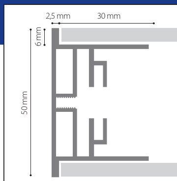
DOUBLE SIDED
