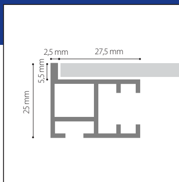
SINGLE SIDED
